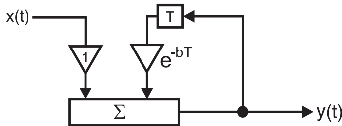
Figure 19: IIR filter
